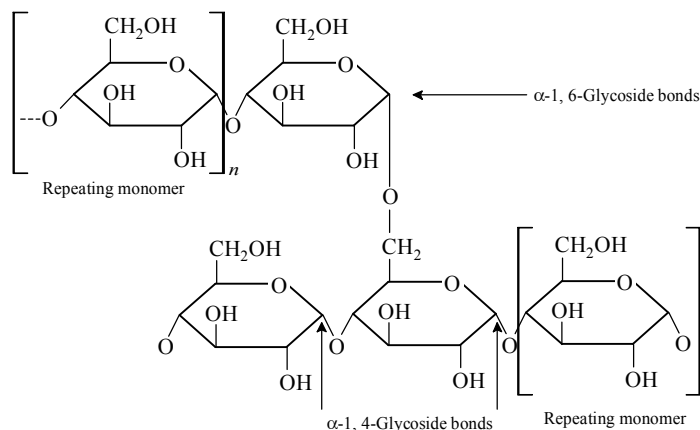
Structure of amylopectin
