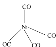
Tetracarbonyl nickel (0) \text{Ni(CO)}_4
