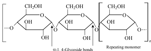
Structure of amylose
