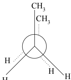
Fully eclipsed (most unstable)
