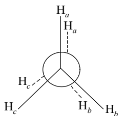
Eclipsed form (least stable)
