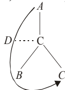
S -Configuration
