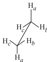
Staggered form (Most stable)
