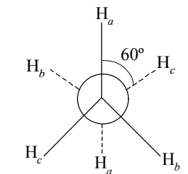
Staggered form (most stable)
