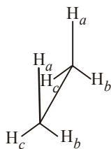
Eclipsed form (Least stable)
