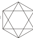
Octahedral void
