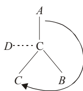
R -Configuration
